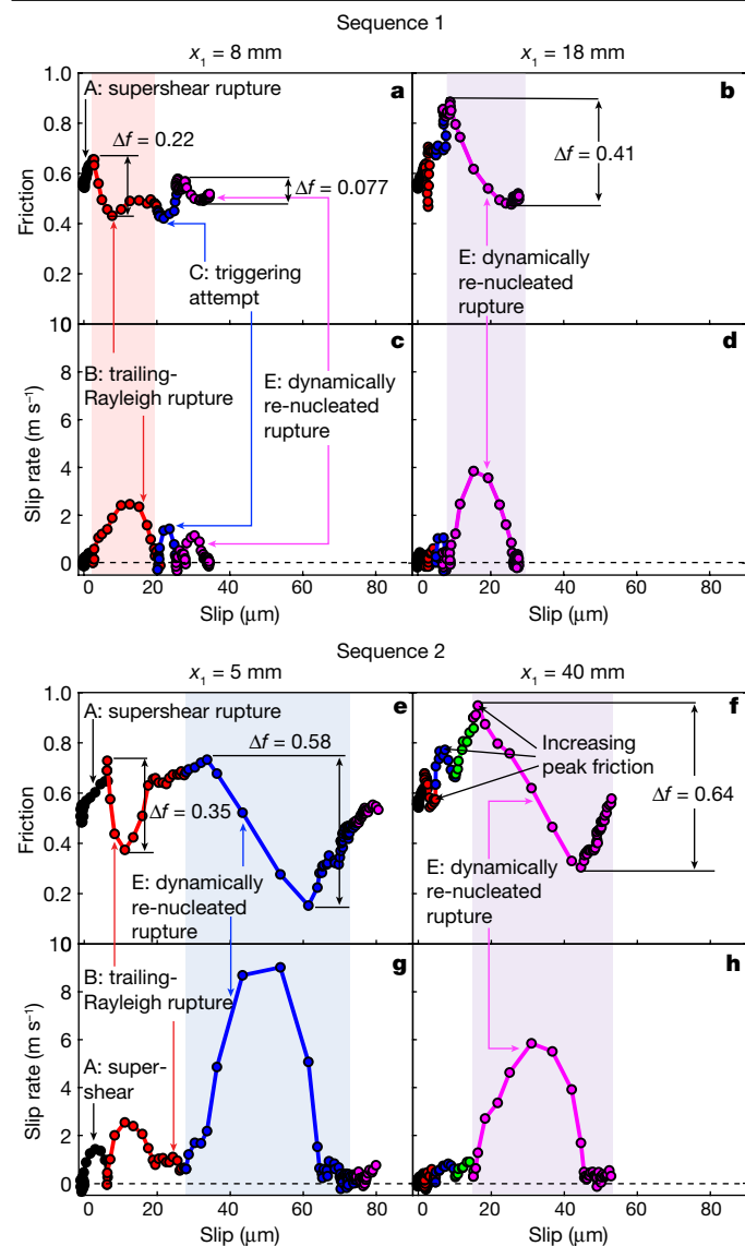
Fig. 4 | Evolution of dynamic friction within the rock gouge with repeated strengthening, pronounced weakening and healing. a–h. Friction versus slip (a, b, e, f) and slip rate versus slip (c, d, g, h) for the rupture sequences 1 (a–d) and 2 (e–h), for selected locations along the interface. The friction evolution in both sequences is characterized by marked strengthening, for slip rates as high as 0.5–2 m s -1 , followed by dramatic weakening at higher slip rates consistent with flash heating. It is noted that strengthening and weakening occur over comparable slip scales of 5–30 μm (see also Extended Data Fig. 10) and, together, explain the intermittent rupture arrest and re-nucleation.
