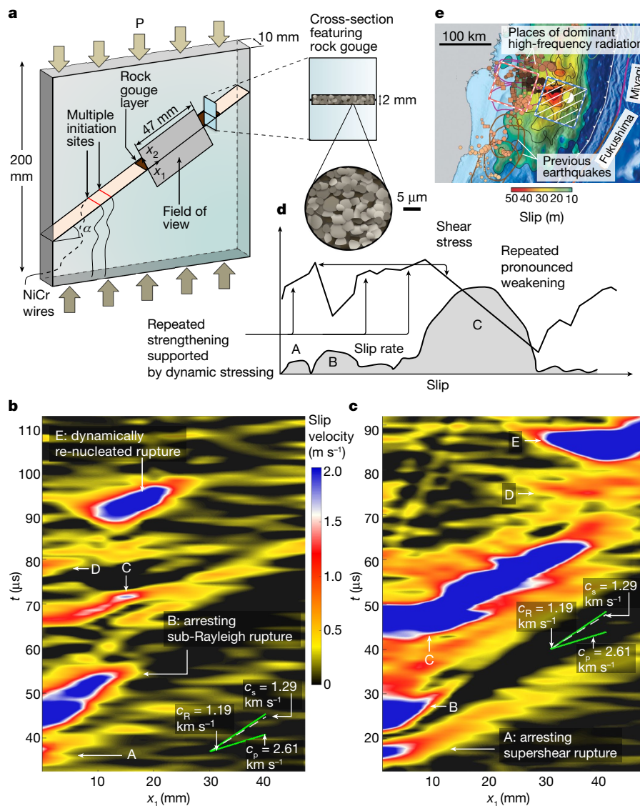
Fig. 1 | Intermittent lab earthquake rupture sequences in rock gouge.
