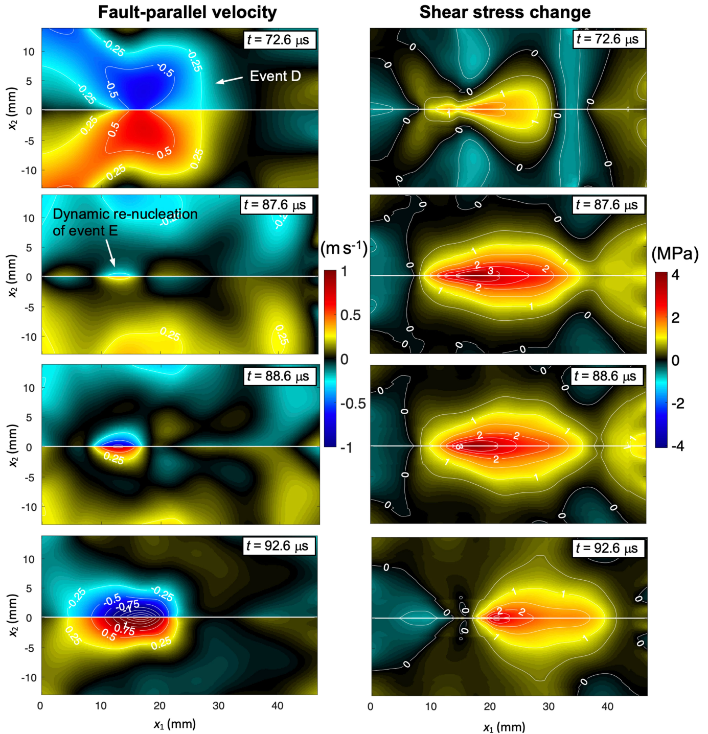
Extended Data Fig. 4 | Snapshots of the full-field distributions of fault-parallel particle velocity and shear stress change during the later phase of the first rupture event. The full-field maps of the propagation of a triggering attempt (event D) at t = 72.6 \mu\text{s} (top row) indicate that, even at this intermediate time between the arrest of event B at 56.6 \mu\text{s} (Extended Data
